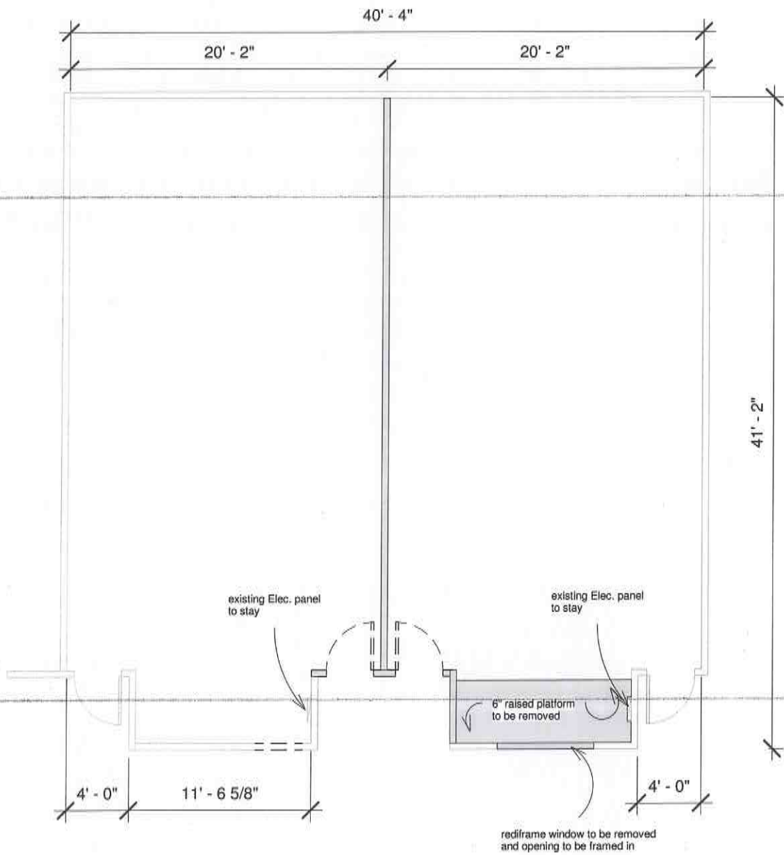
1 Demo Plan 1/8" = 1'-0"
